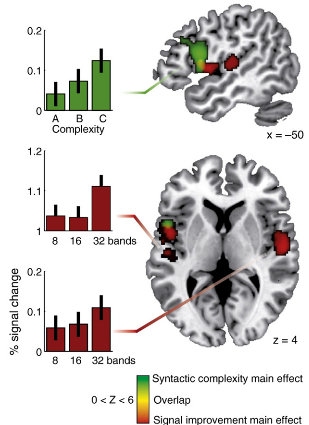
Fig. 3. Activation overlays from Experiment 2 for the main effects of syntactic complexity (shown in green) and signal improvement (shown in red). All activations are thresholded at p<0.001 and a minimum cluster size of 41 supra-threshold voxels to control for family-wise error at p<0.05 . A small overlap of the main effects is seen in the left inferior frontal cortex (shown in yellow). Note that the posterior STS activation “cancels out” in the main effect of complexity, as Figs. 5 and 6 show how activation there is shifted as an interaction of complexity and degradation. Note that error bars have been corrected to reflect within-subject error (Jarmasz and Hollands, 2009).
