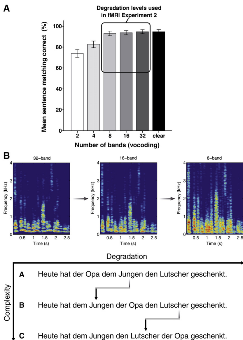
Fig. 2. A. Results of the behavioral pilot experiment to Experiment 2. The mean percentage of correct sentence matching is shown for 2- to 32-band vocoded and clear speech. From 8-band on, scores do not differ significantly from each other (clear speech; rightmost bar). Thus, we chose vocoding with 8, 16, and 32 bands (lower panels) for fMRI Experiment 2. B. Example stimuli for Experiment 2 (increasing in syntactic complexity from top to bottom). All sentences literally translate as “today the grandfather has given the lollipop to the boy.” For Experiment 2, acoustically degraded versions were additionally introduced, as exemplified by the spectrograms with spectral detail declining from left (32-band speech, almost clear speech) to right (8-band speech, moderately degraded speech).
