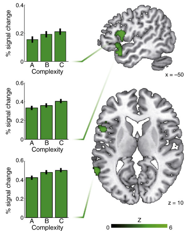
Fig. 1. Effect of increasing syntactic complexity in Experiment 1. All activations are thresholded at p < 0.001 and a minimum cluster size of 41 suprathreshold voxels to control for family-wise error at p < 0.05 . Bar graph panels show % signal change from the parametric syntactic complexity contrast for the left IFG (henceforth referred to as pars opercularis , PO) in panel 1 and two regions of the superior temporal cortex (BA 13 in panel 2 and BA 22 in panel 3). Note that error bars have been corrected to reflect within-subject error (Jarmasz and Hollands, 2009).
