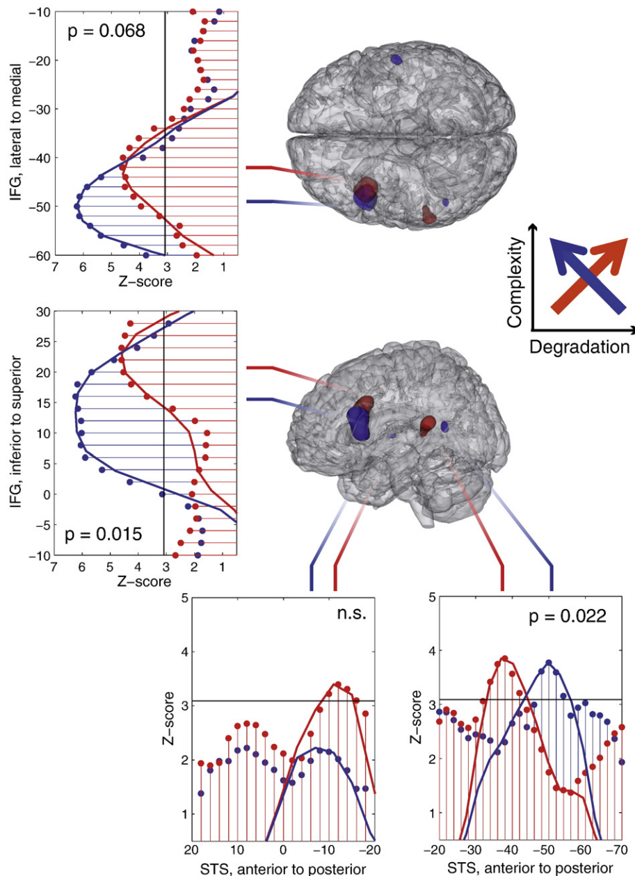
Fig. 6. Coordinate shifts for Experiment 2 (“upstream delegation”). The activation overlays and maximum Z-score per coordinate plot illustrate the syntactic complexity activation cluster in the IFG and STS sites shift from signal improvement toward signal degradation (i.e., blue to red). Parametric trade-off between syntactic complexity and signal improvement (blue) drives more inferior and lateral left IFG (left panels) and more anterior and posterior left STS sites (bottom panels). P-values indicate the significance of two-sample Cramér–Von Mises tests run on the indicated spatial distributions. Parametric additivity of syntactic complexity and signal degradation activates a more medio-dorsal prefrontal site (left panels) and more middle STS sites (bottom panels). Linear contrasts that yielded these patterns are schematized with arrows in the coordinate system.
