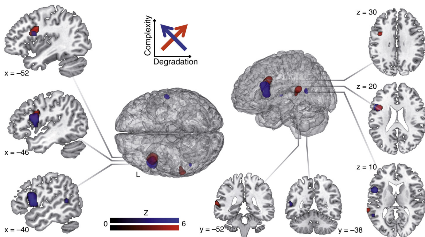
Fig. 5. Effects of increasing syntactic complexity under varying acoustic degradations in Experiment 2. The panels show activation overlays of the two major contrasts: increasing syntactic complexity trading off with signal improvement (blue); and increasing syntactic complexity additive to signal degradation (red). See Table 2 for exact contrast formulation. All activations are thresholded at p < 0.001 and a minimum cluster size of 41 supra-threshold voxels to control for family-wise error at p < 0.05 . Linear contrasts that yielded these patterns are schematized with arrows in the coordinate system.
