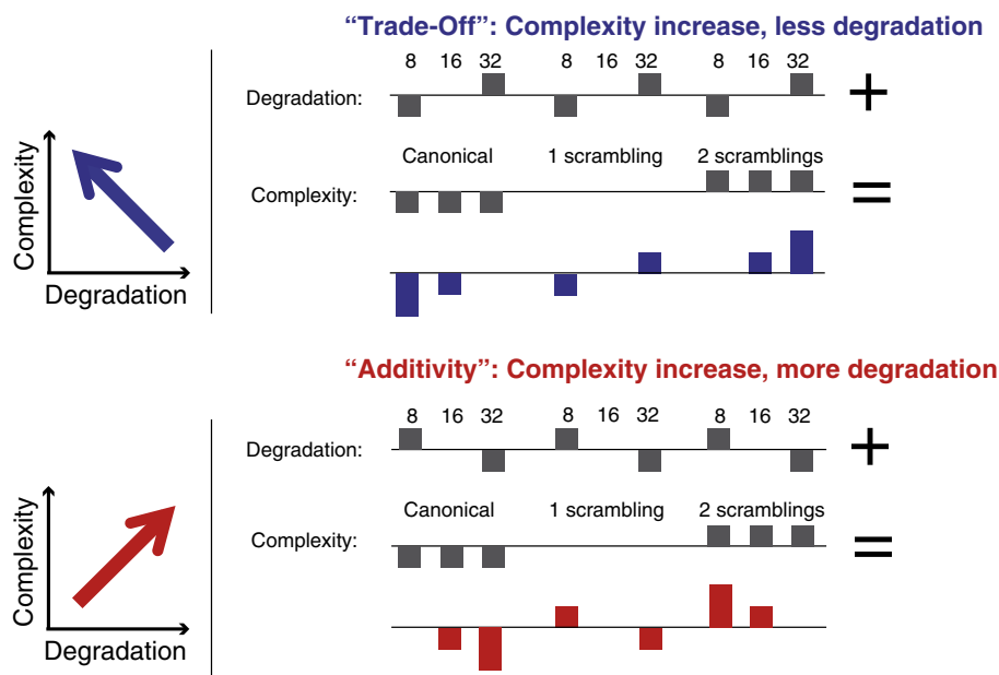
Fig. 4. Contrast design for additivity and trade-off. Schematic display of the linear contrasts formulated for testing “additivity” (i.e., increasing syntactic complexity adds up with signal degradation, leading to the strongest activation at 8-band/two-scramblings speech; shown in red) and “trade-off” (i.e., increasing syntactic complexity trades off with signal degradation, leading to the strongest activation at 32-band/two-scramblings speech; shown in blue).
